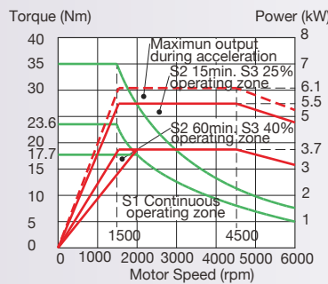
A200 (BMT-55)
