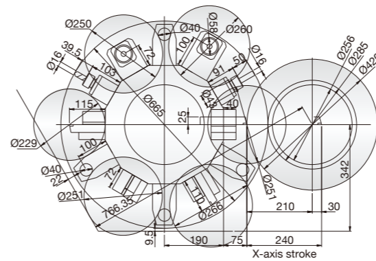
Vturn-S36
