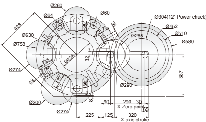
Vturn-S36CM
