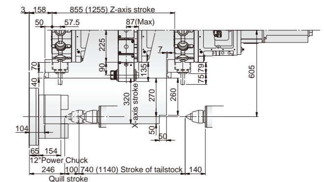
Vturn-S36/85 (S36/125)
