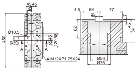
BMT-75 (Vturn-S36CM)
