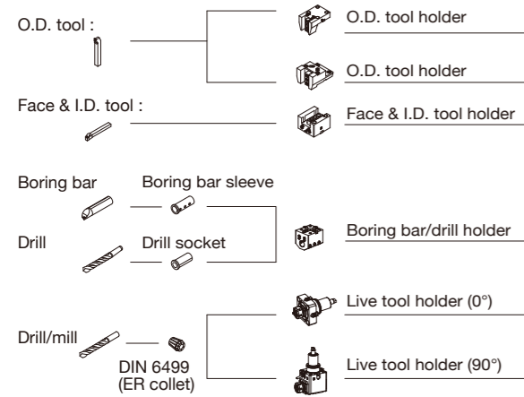
BMT-55 (Vturn-S20CM)
