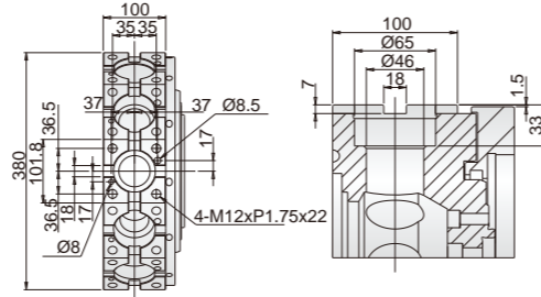
BMT-65 (Vturn-S26CM)
