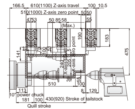
Vturn-S26/60 (S26/110)
