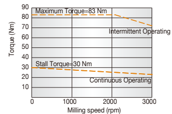
αiF 30/4000 (7 kW)
