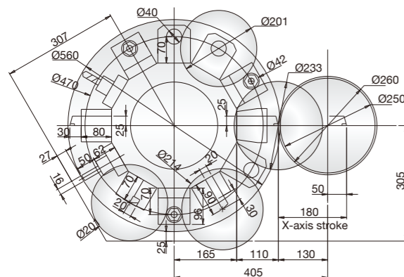
Vturn-S20CM
