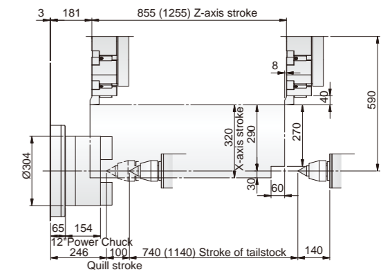
Vturn-S26/60 (S26/110)
