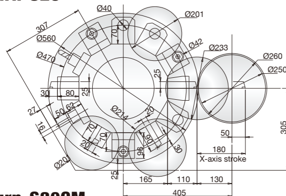
Vturn-S20CM
