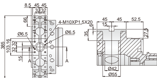
BMT-55 (Vturn-S20CM)
