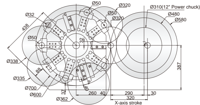
Vturn-S36
