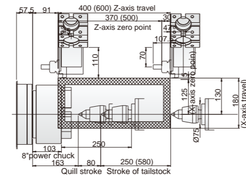
Vturn-S20/40 (S20/60)
